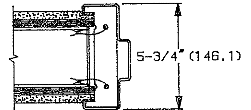
TRUSS STEEL STUD WITH PLASTER ON ROCK LATH
